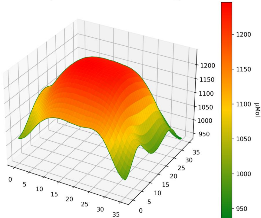
PPFD 3D Heatmap LT-5840 - LIGHTNING Basic EVO @600mm
